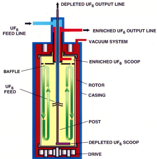
SCHEMATIC DIAGRAM OF A GAS CENTRIFUGE
